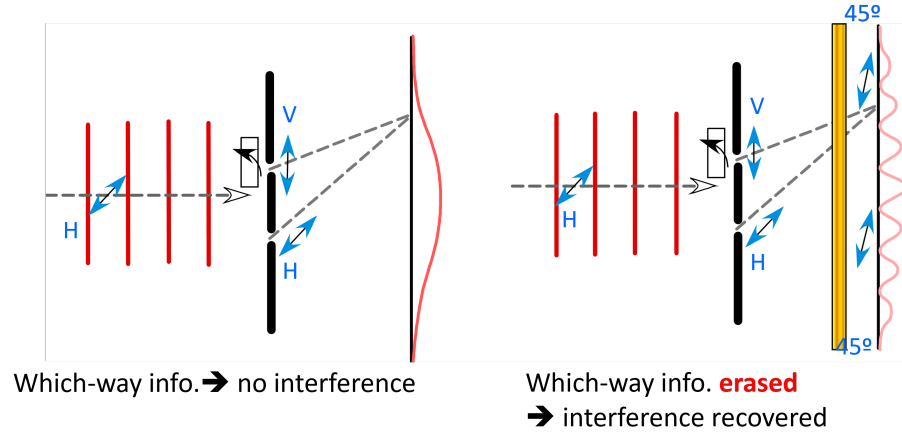
FIG. 4. Illustration of the which-way information in the double-slit experiment.
